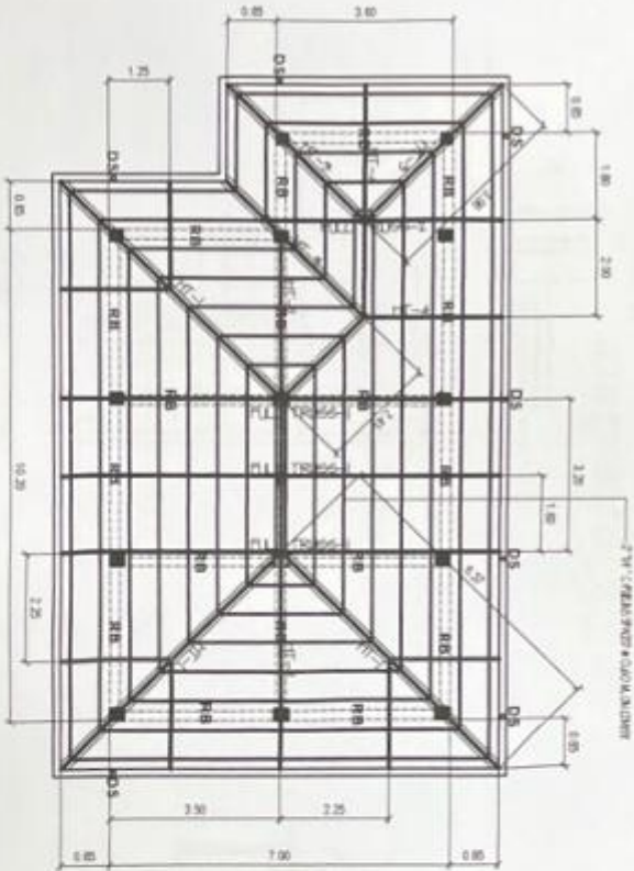
STEEL TRUSSES DIAGRAM SCALE 1:50 METERS
