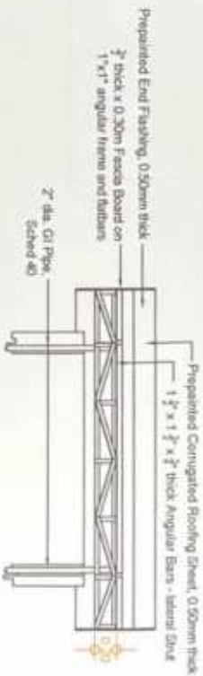
LATERAL STRUT Scale 1:50
