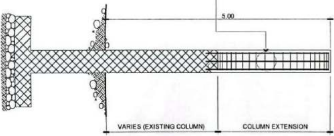
DETAIL OF COLUMN (C1) SCALE 1:500
