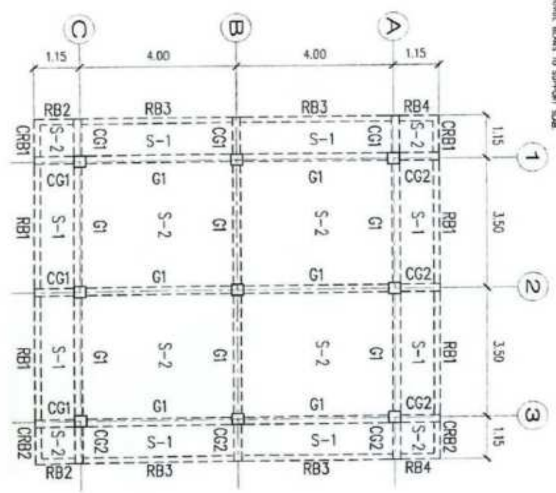
ROOF DECK PLAN SCALE 1:100M
