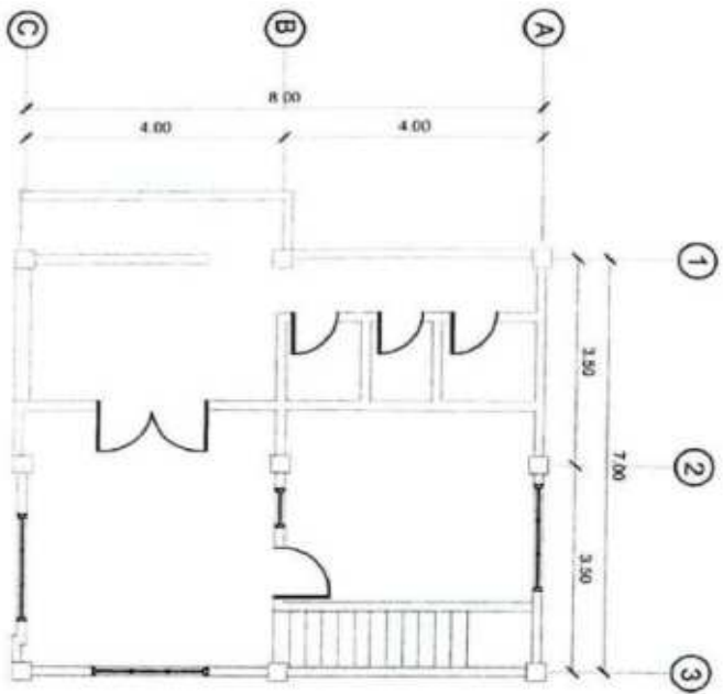
EXISTING GROUND FLOOR PLAN SCALE 1:100MMTS
