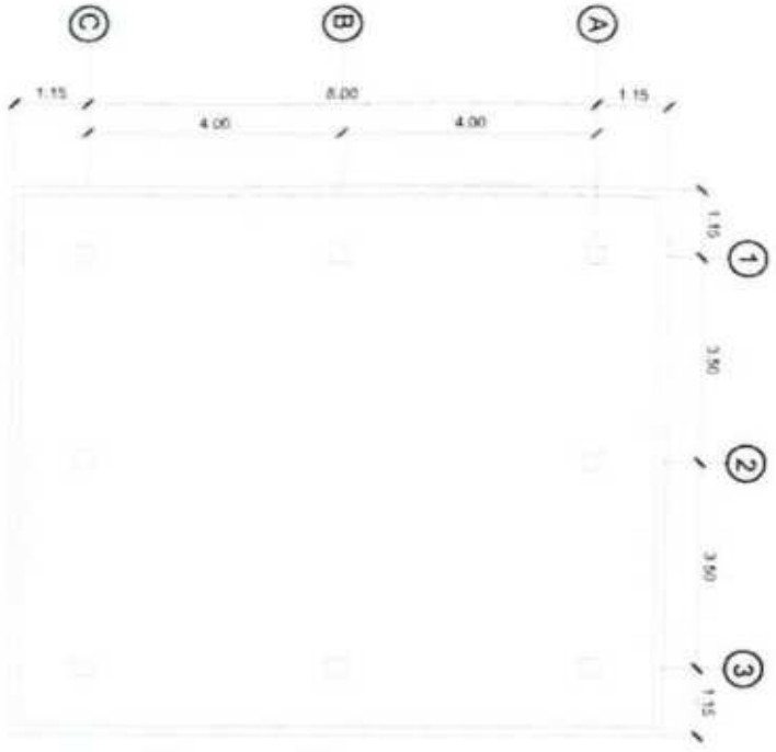
PROPOSED ROOFDECK PLAN SCALE 1:100/MPTS
