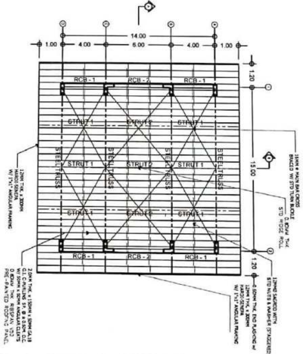
ROOF FLAMING PLAN SCALE: 1:200 METERS
