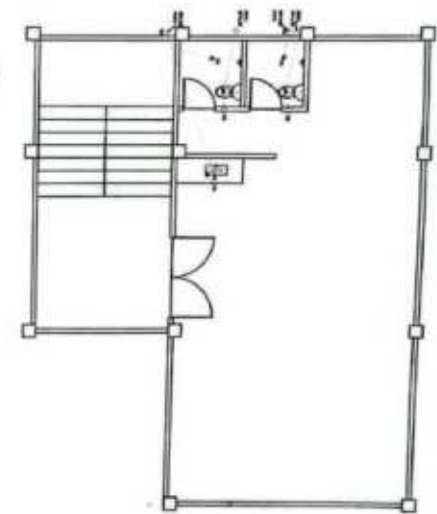
SECOND FLOOR SANITARY LAYOUT SCALE 1:1000
