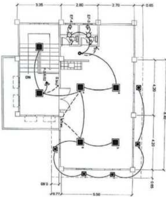
LIGHTING LAYOUT - SECOND FLOOR SCALE 1:1000
