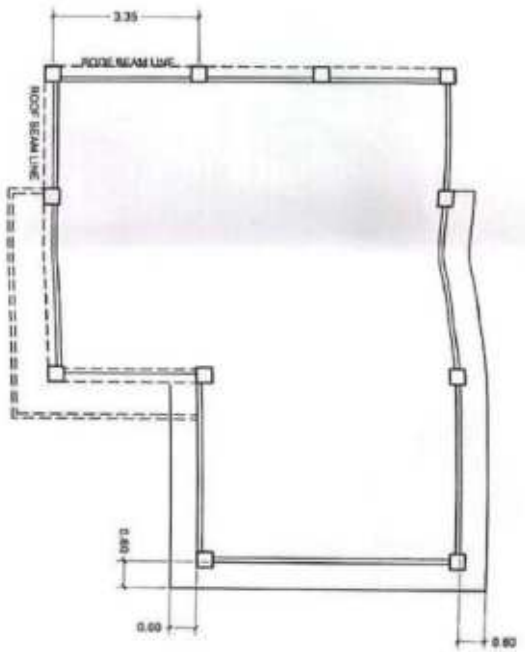
ROOF DECK PLAN SCALE 1:1000
