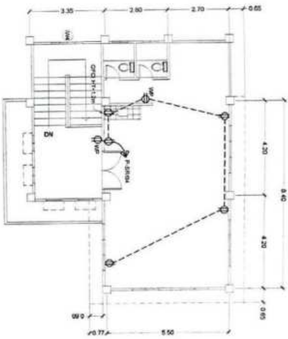
POWER LAYOUT - SECOND FLOOR SCALE 1:100M
