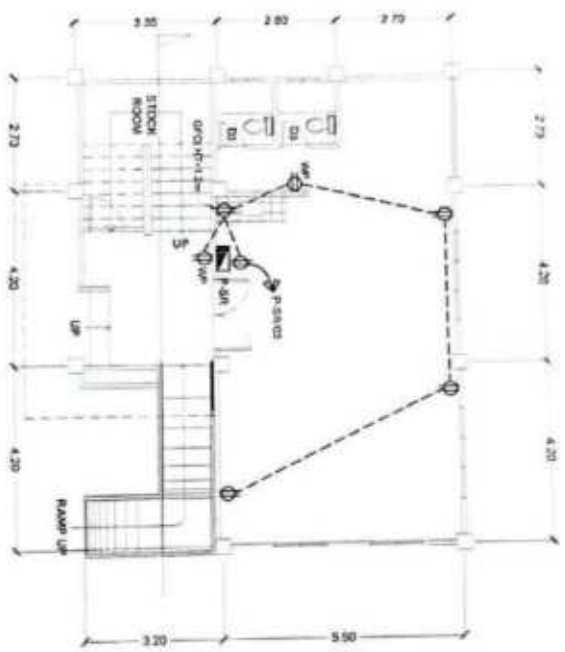
POWER LAYOUT - GROUND FLOOR SCALE 1:500M
