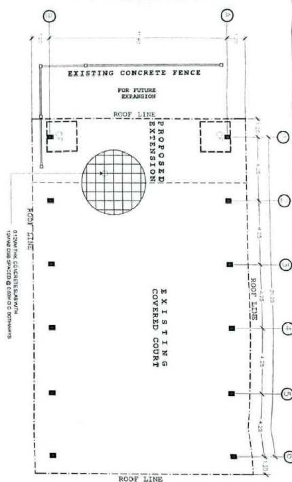
FOUNDATION PLAN SCALE 1:150 METERS
