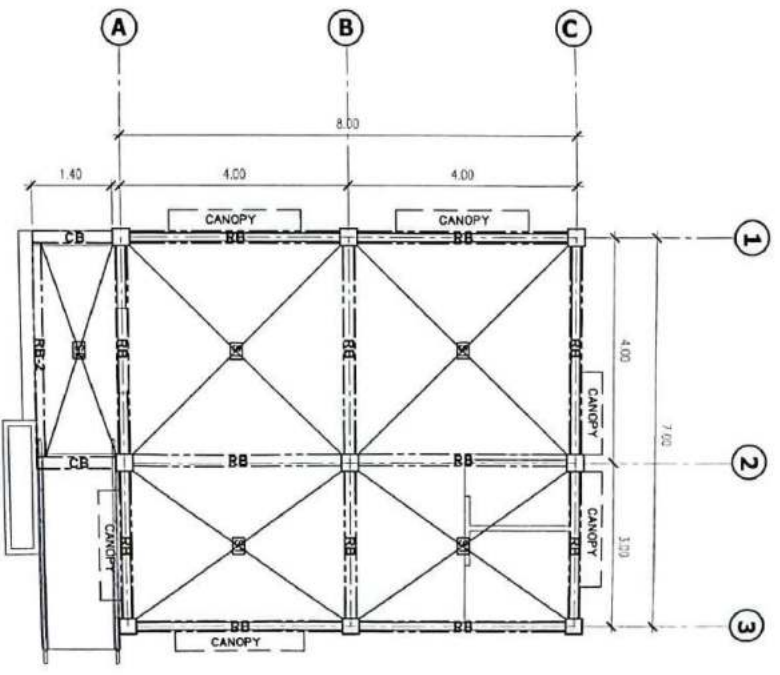
ROOF FRAMING PLAN SCALE 1:80 MTS
