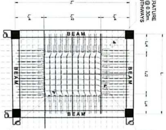
DETAIL OF SLAB NTS
