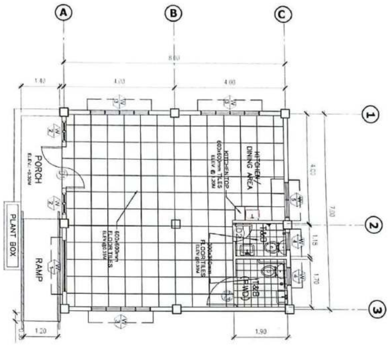
GROUND FLOOR PLAN SCALE 1:80 MTS
