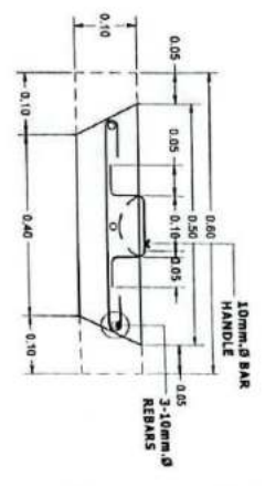
DETAILS OF MANHOLE SCALE 1:50 MTS
