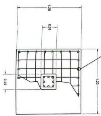
DETAILS OF COLUMN FOOTING SCALE 1:100 MTS
