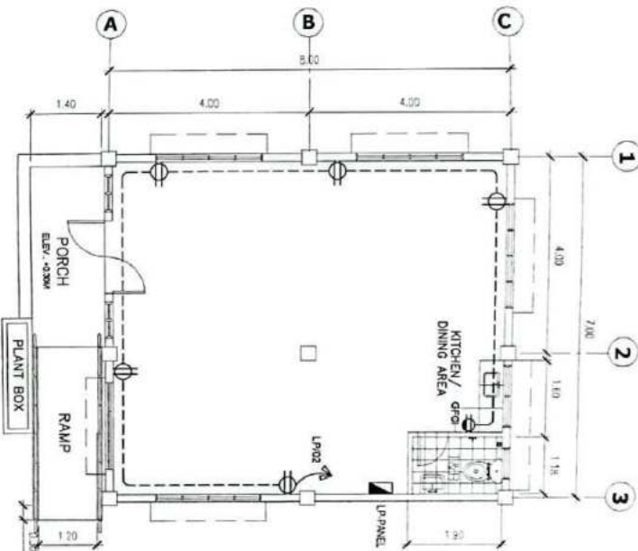
GROUND FLOOR PLAN SCALE 1:80 MTS
