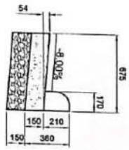
DETAIL OF CONCRETE CURB AND GUTTER SCALE 1:10
