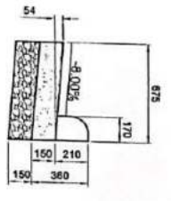
DETAIL OF CONCRETE CURB AND GUTTER SCALE 1:10
