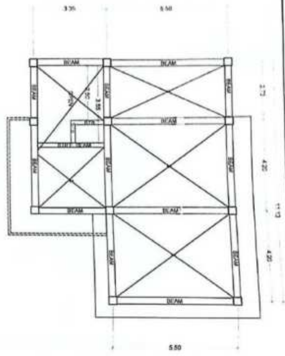
2ND FLOOR BEAM SCALE 1/1000
