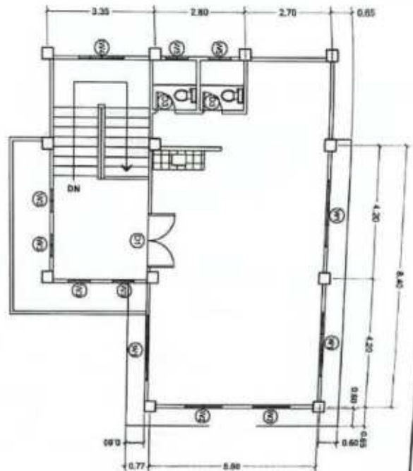
2ND FLOOR PLAN SCALE 1:1000
