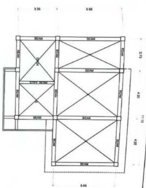
ROOF BEAM SCALE 1/1000
