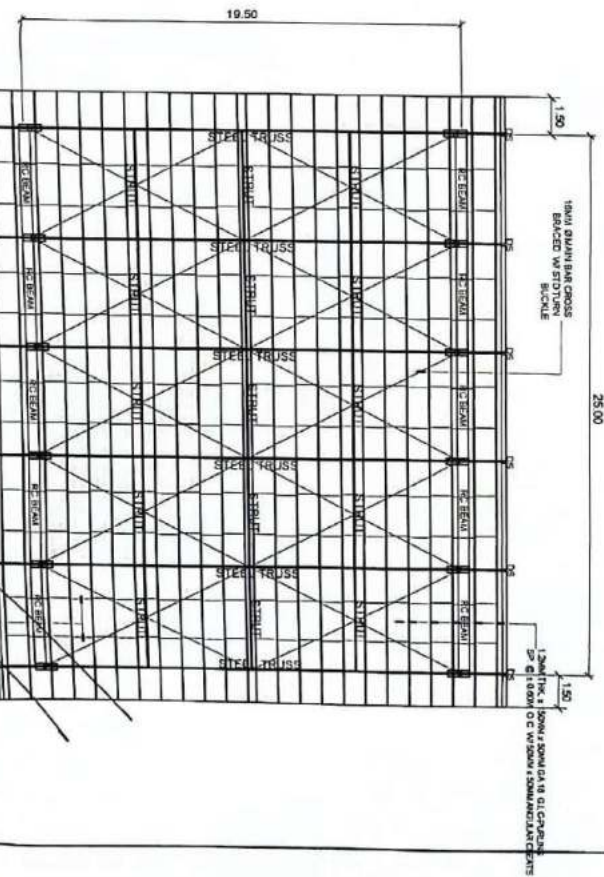
ROOF FRAMING PLAN SCALE: 1:200 METERS
