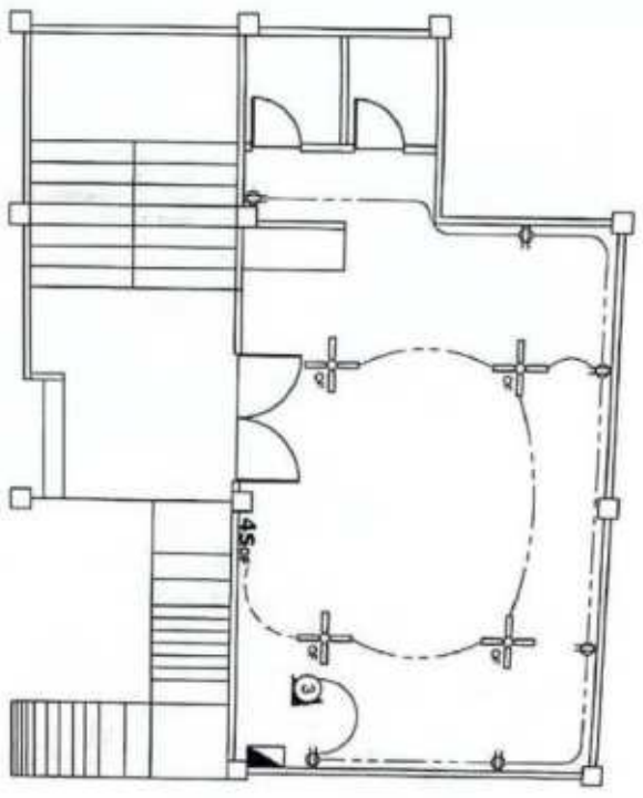
SCALE GROUND FLOOR POWER LAYOUT SCALE 1:100M/TS
