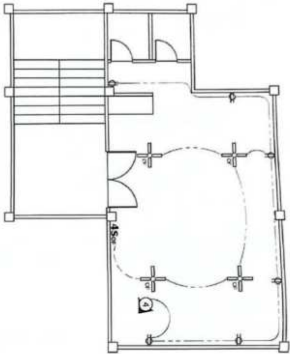
SECOND FLOOR POWER LAYOUT SCALE
