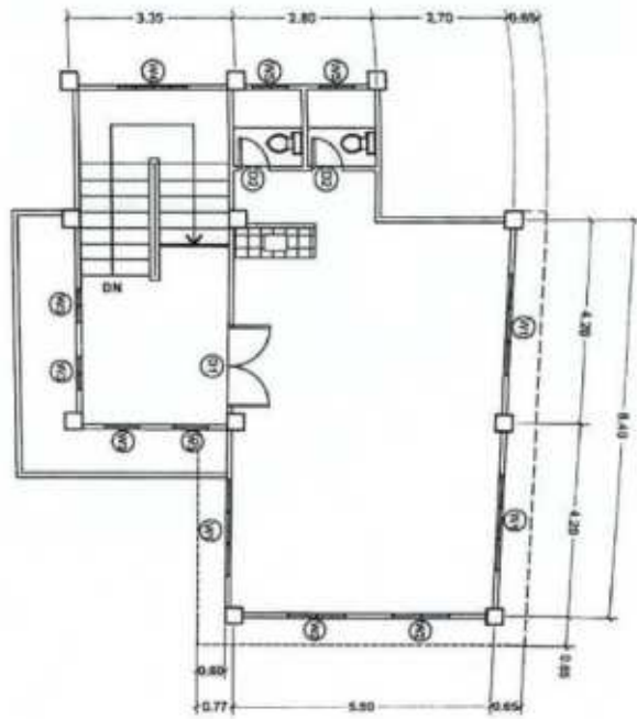
SECOND FLOOR PLAN SCALE 1:1500
