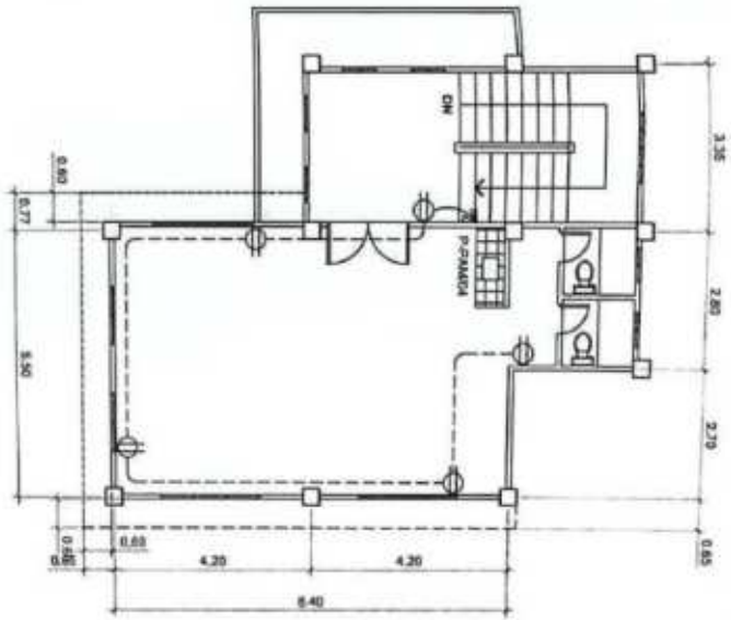
2ND FLOOR PLAN SCALE 1:100MM
