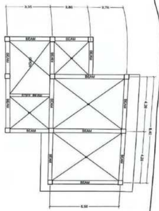
ROOF BEAM SCALE 1:100M
