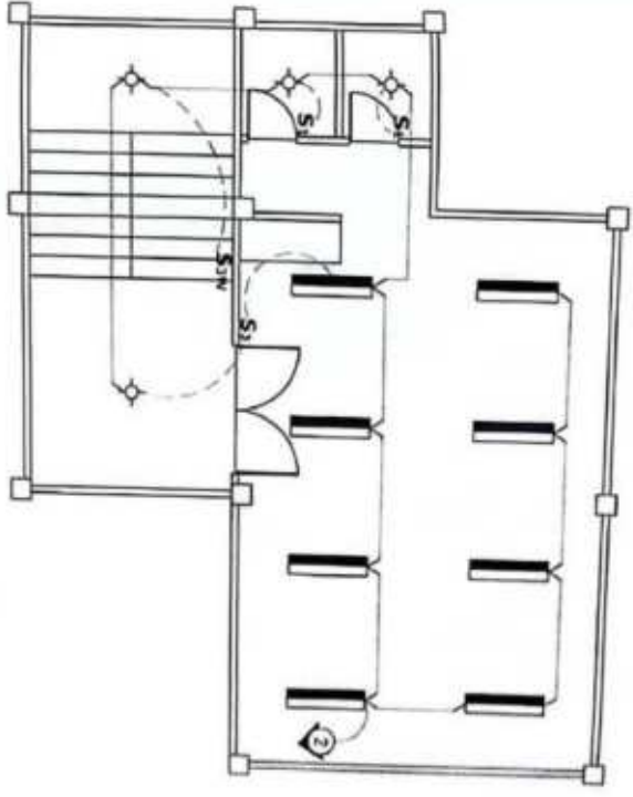
SECOND FLOOR LIGHTING LAYOUT SCALE 1:100METS
