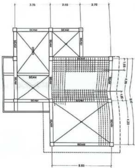
SECOND FLOOR BEAM SCALE 1:100M
