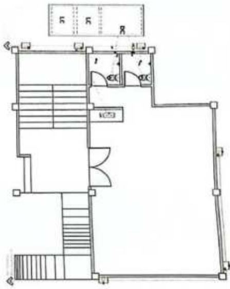
GROUND FLOOR SANITARY LAYOUT SCALE 1/8"=1'-0"
