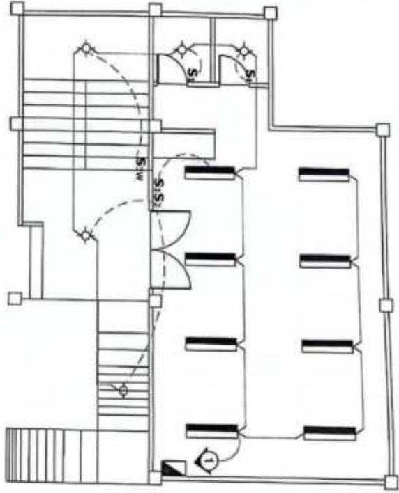
GROUND FLOOR LIGHTING LAYOUT SCALE 1:100METS
