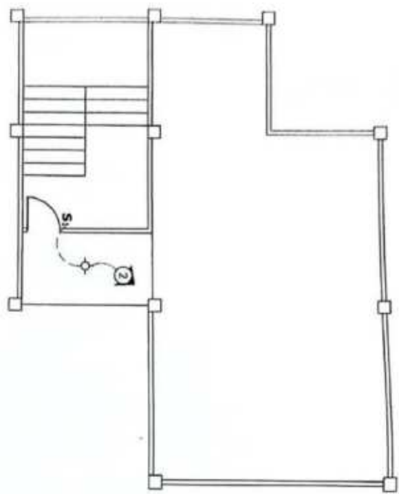
SCALE ROOF DECK LIGHTING LAYOUT SCALE 1:100M/TS
