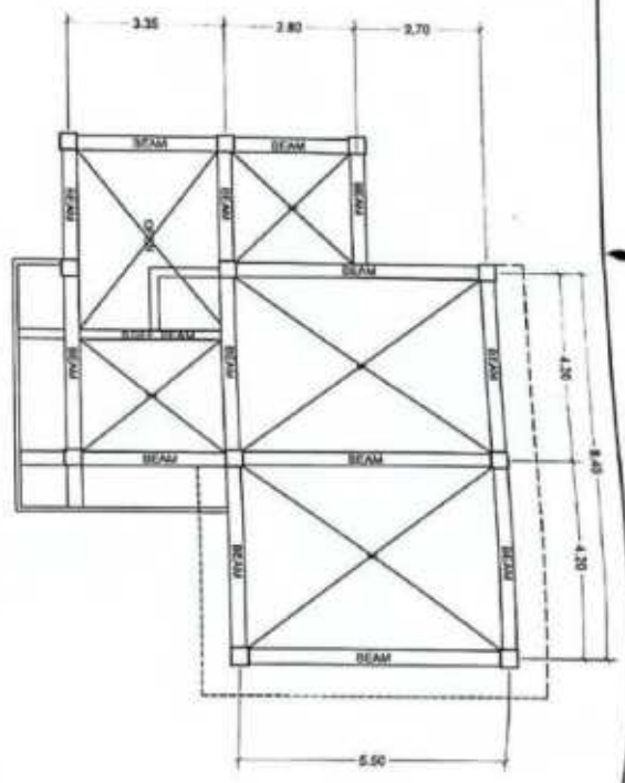
2ND FLOOR BEAM SCALE 1:100M
