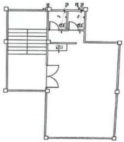
SECOND FLOOR SANITARY LAYOUT SCALE 1/8"=1'-0"
