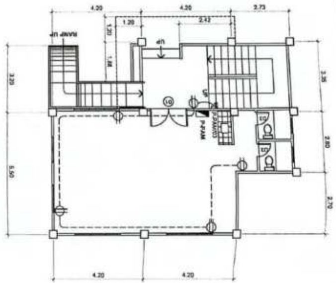
GROUND FLOOR PLAN SCALE 1:100MM
