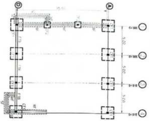
FOUNDATION PLAN 11
