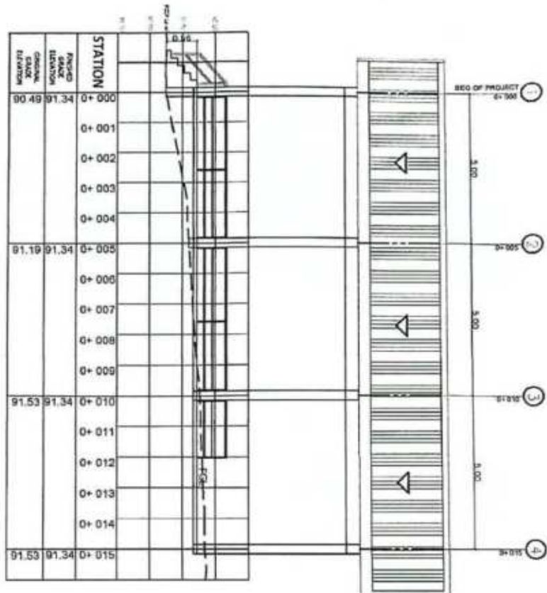
ELEVATION PROFILE DETAIL
