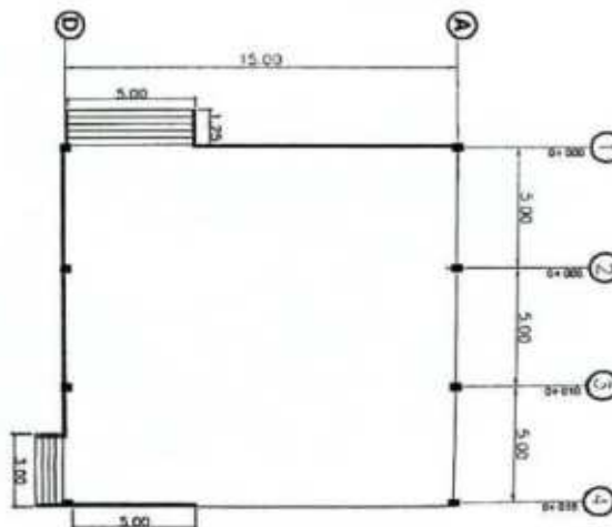
FLOOR PLAN SCALE: 1:200 (METERS)
