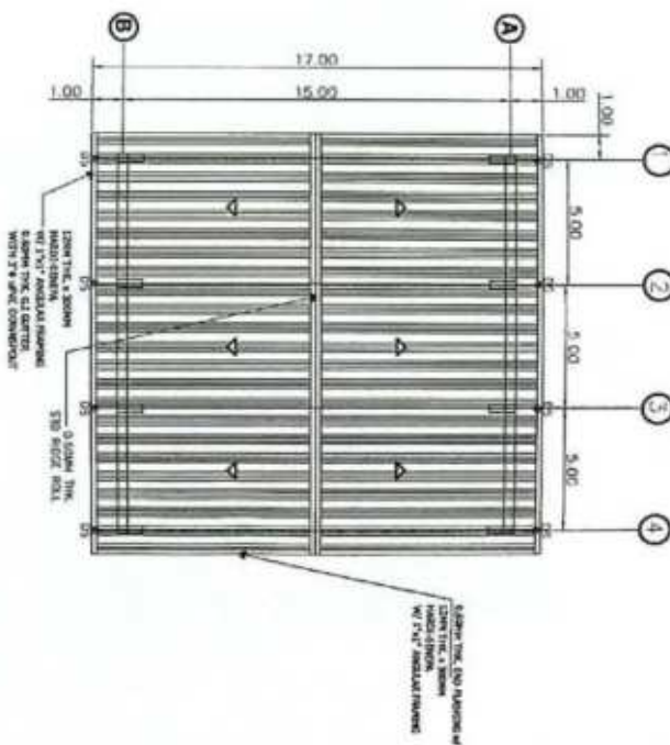
ROOF TINNING PLAN SCALE: 1:200 METERS
