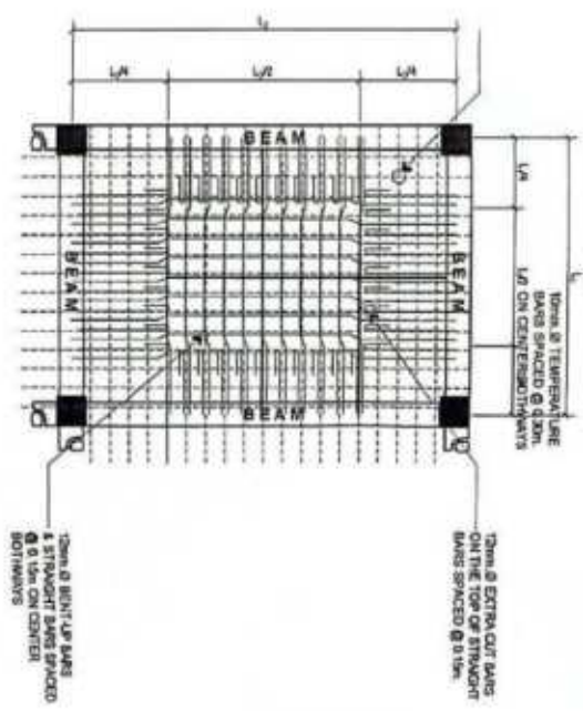
DETAIL OF SLAB NTS
