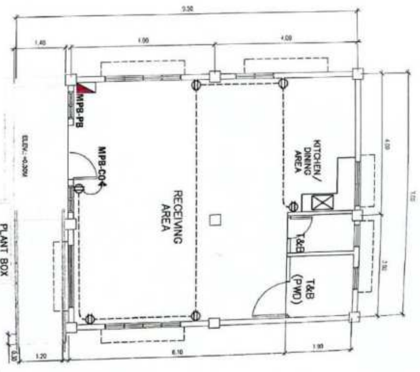
POWER LAYOUT SCALE 1:50 MTS
