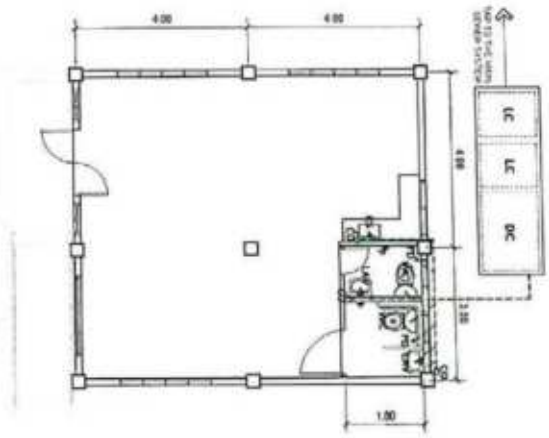
SEWER LAYOUT PLAN SCALE 1:100 M.T.S
